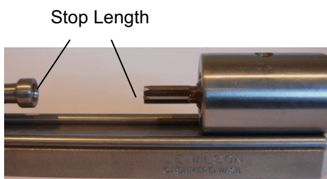
Neck Reamer Shown In Case Trimmer
